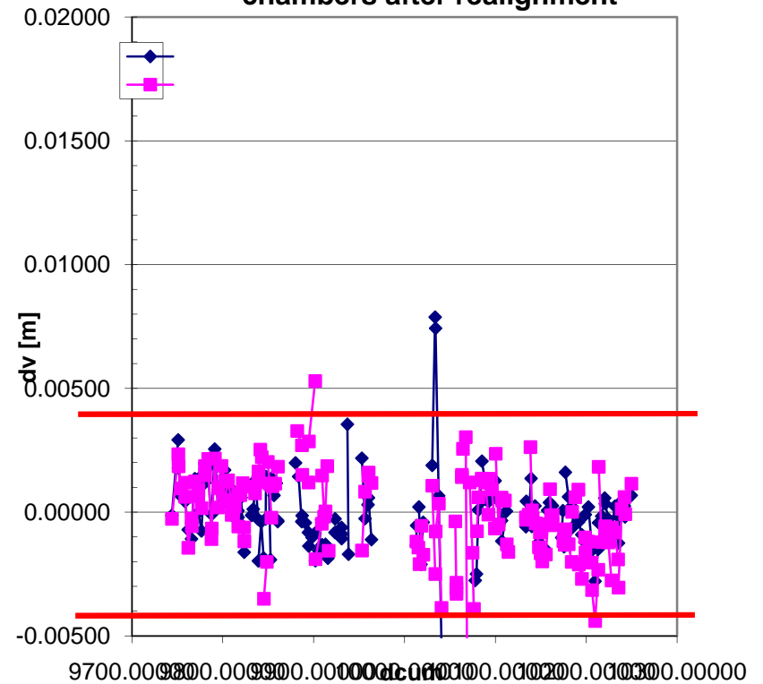
LSS4 vertical position of vacuum chambers after realignment
