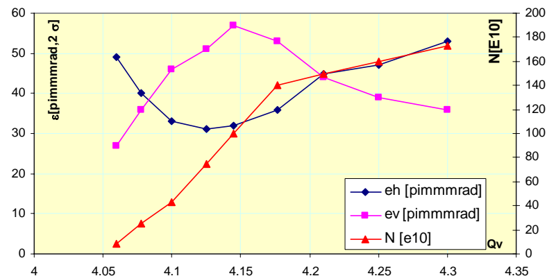
emittances versus vertical tune
