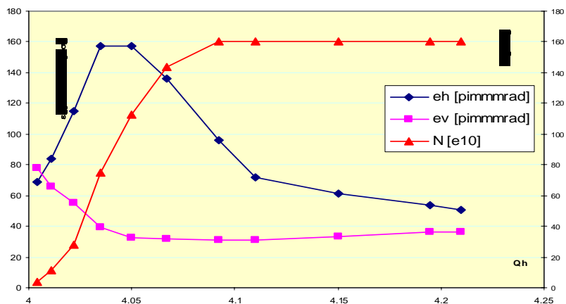
emittances versus horizontal tune
